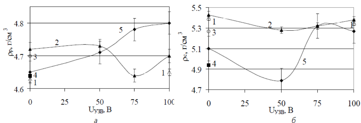
Fig. 1. The density of compressions p - (a) and sintered BTCII ceramics p - (b) depending on the intensity of ultrasound and pressure of pressing ( P ) \gamma\text{ДП} BTCII: 1) 746 MPa; 2) 907 MPa; 3) 1069 MPa; and the charge of standard reagents: 4) 746 MPa; 5) 907 MPa
