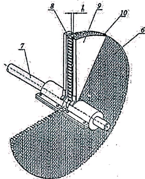
Figure 8. Axonometric view of the insulating chamber
