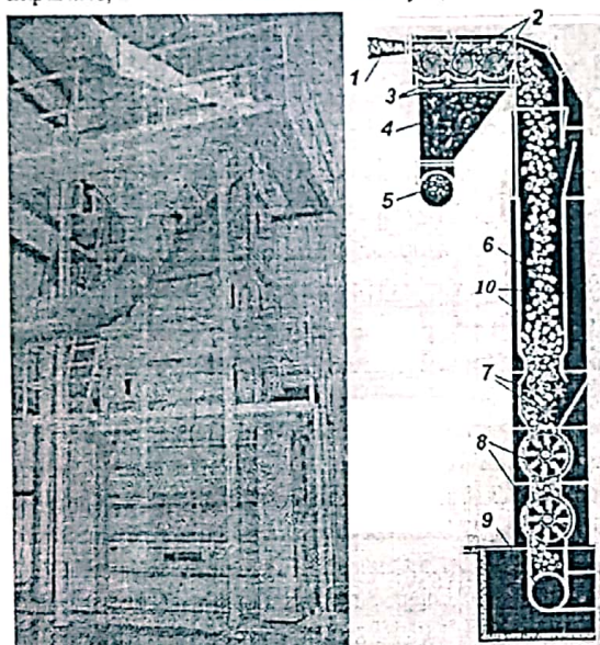
Figure 4. The technological scheme and appearance of the Separator Big "J"
