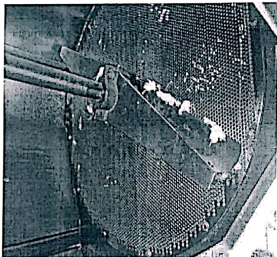
Figure 10. Appearance of the inner separator of the improved separator
