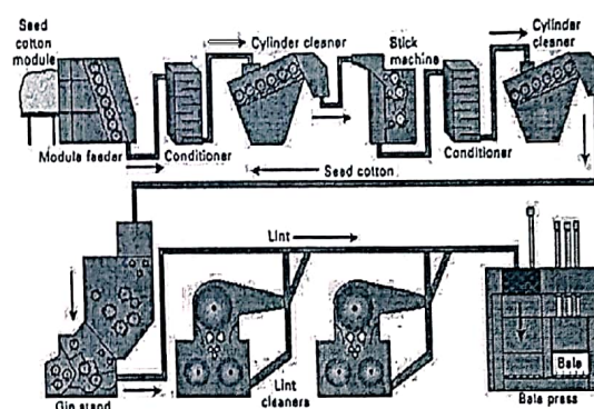
Figure 2. Modern foreign technological process in cotton processing
