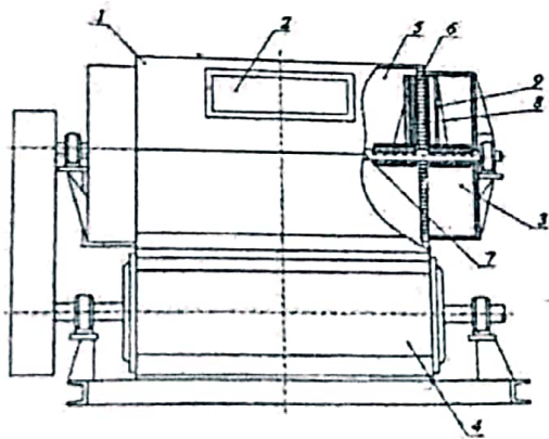
Figure 6. An overview of the new fixture mounted on the improved CC-15A separator
