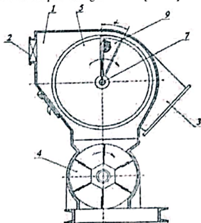
Figure 7. Cross-sectional view of the isolation chamber
